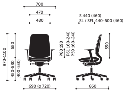
230S / 230SL / 230SFL
