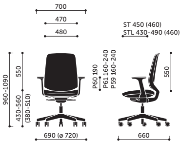
230ST / 230 STL
