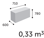
230ST / 230 STL
